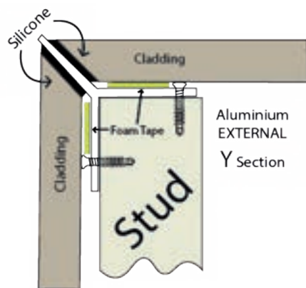
EXTERNAL ALUMINIUM Y SECTION
