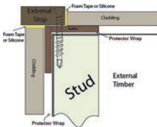
EXTERNAL TIMBER
